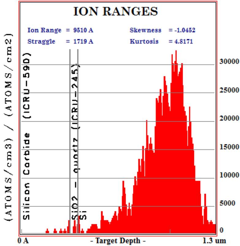
Figure 3.7: Ion Ranges for 1 MeV Ions into SiC(328.5 nm)/SiO 2 /Si
