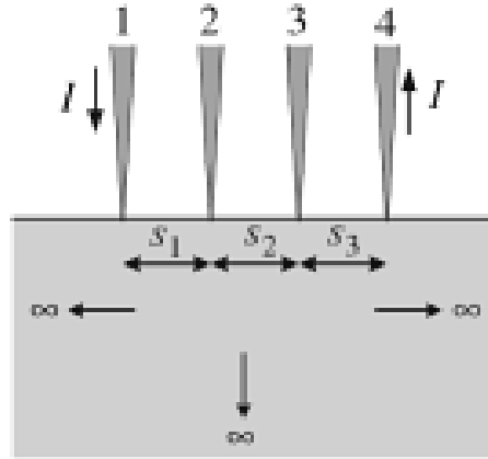
Figure 4.3: Collinear Four Point Probe Illustration
